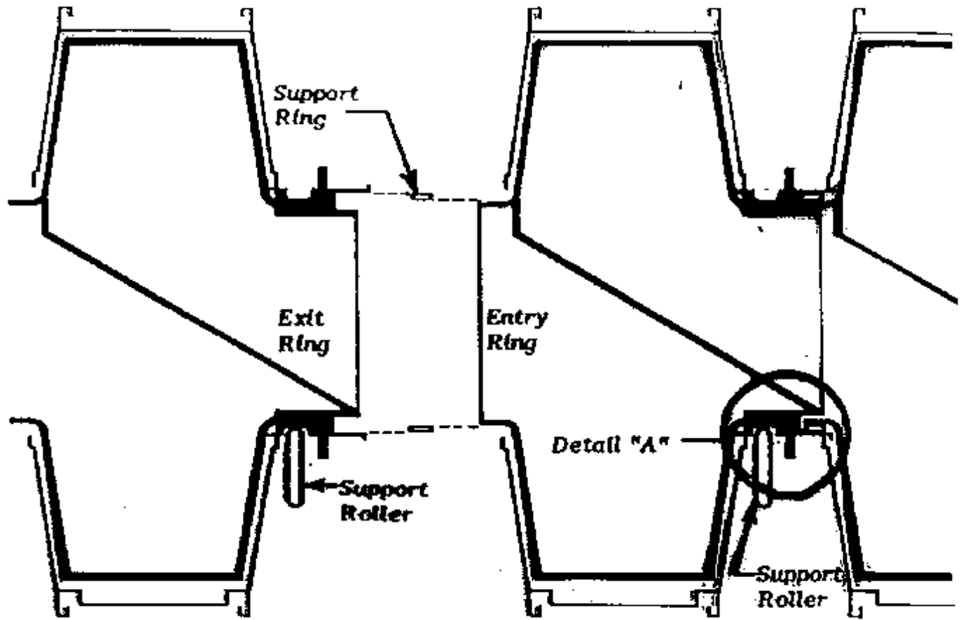
MODULE CROSS SECTION
