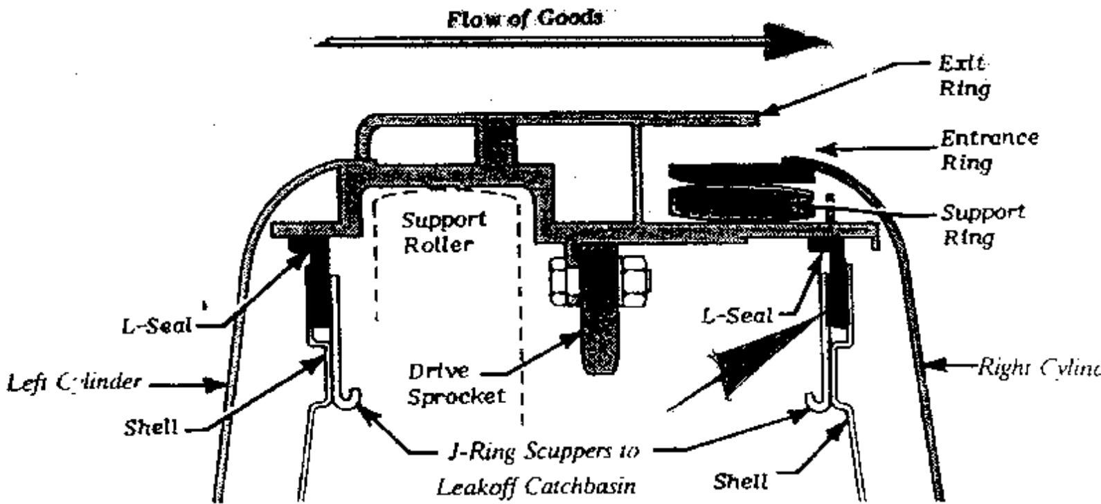
DETAIL "A": INTER-MODULE SEAL
