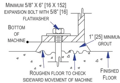
ANCHORING DETAIL
