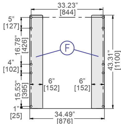
FOUNDATION
