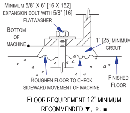
ANCHORING DETAIL
