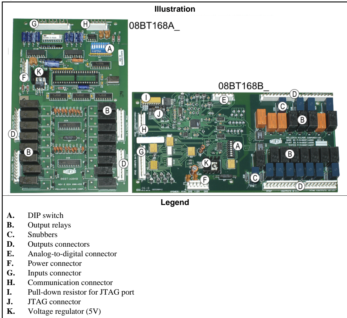
Figure 8: Processor Boards
