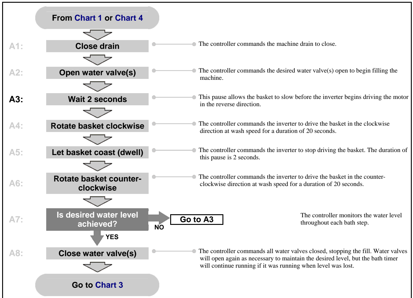
Chart 2: Operating Sequence Part 2
