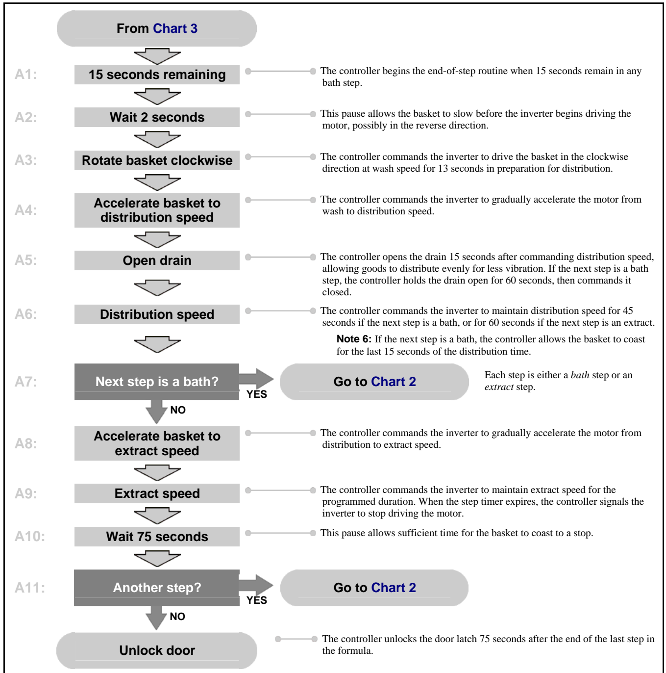
Chart 4: Operating Sequence Part 4
