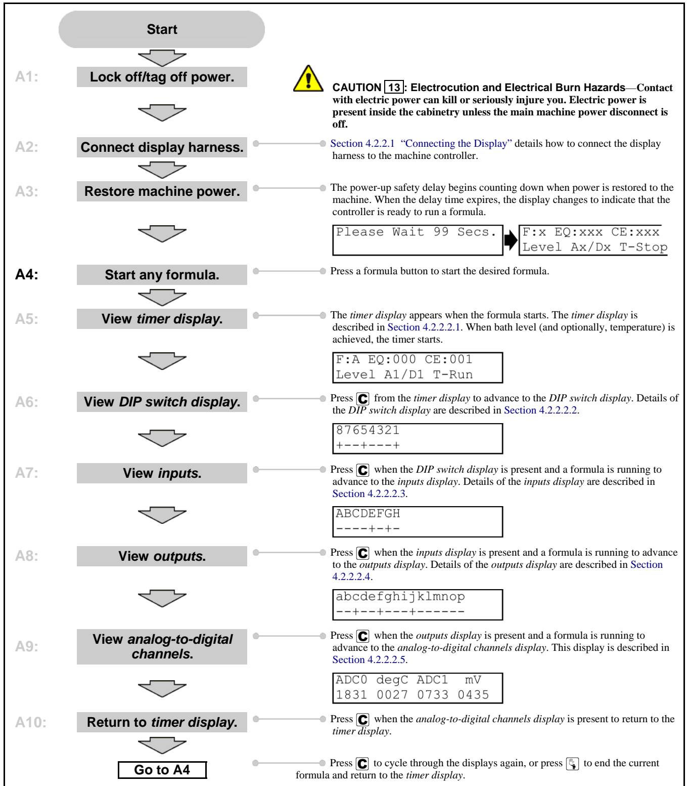
Chart 5: Overview of Run Mode Diagnostics
