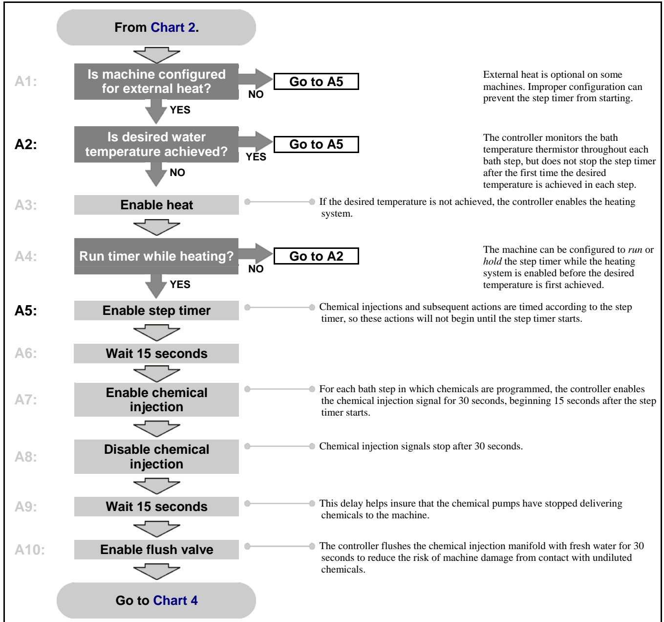
Chart 3: Operating Sequence Part 3
