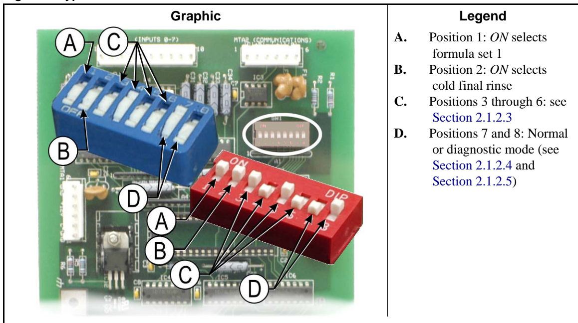
Figure 6: Typical DIP switch on 08BT168AT
