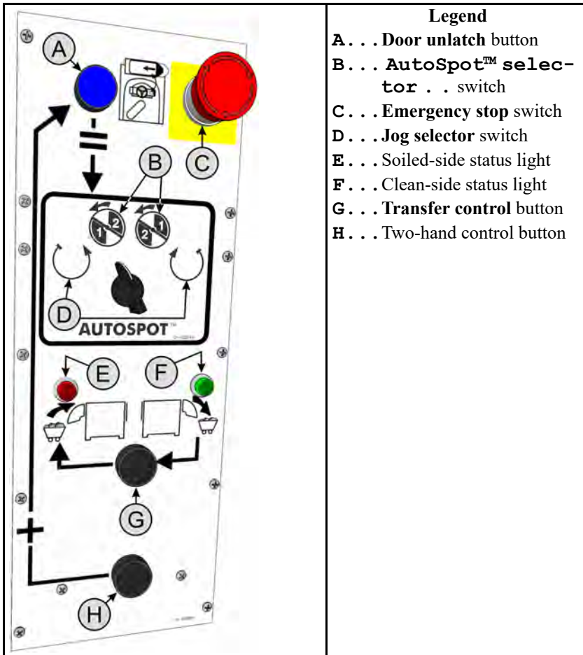
Figure 3. Clean-side Control Panel with Two-pocket AutoSpot™ Selector Switch
