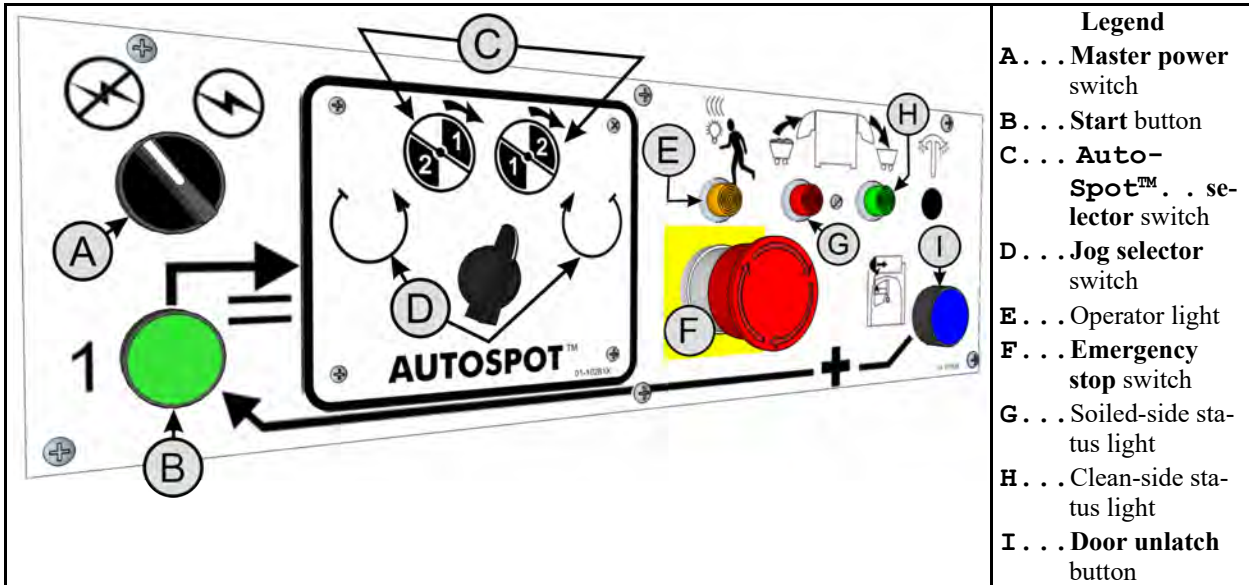
Figure 3. Clean-side Control Panel with Two-pocket AutoSpot™ Selector Switch
