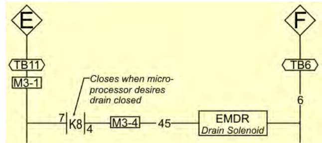
Figure 32. Schematic of Typical Drain Circuit
