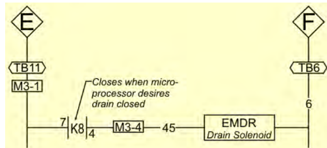
Figure 31. Schematic of Typical Drain Circuit
