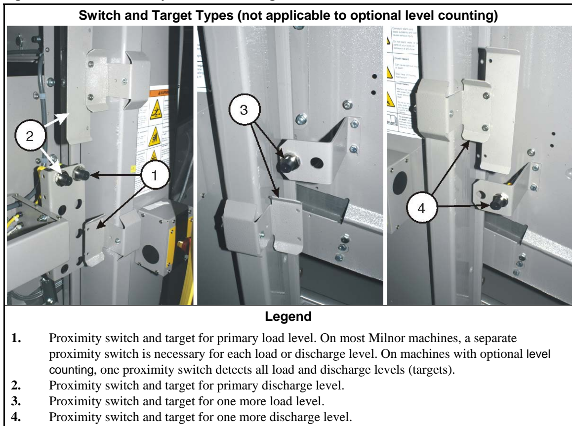
Figure 11: Elevator Proximity Switches and Targets
