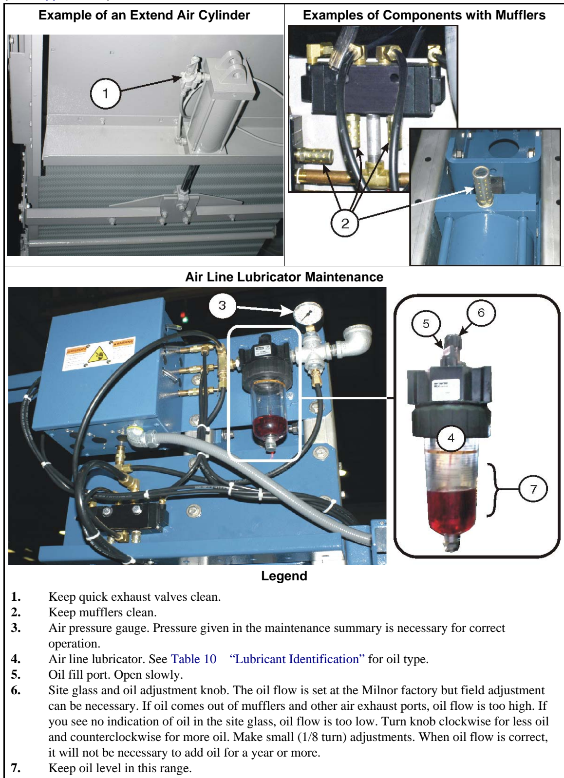
Figure 12: Compressed Air Mechanisms on Wet Goods Shuttles and Some Loose Goods Shuttles (see Supplement 2).
