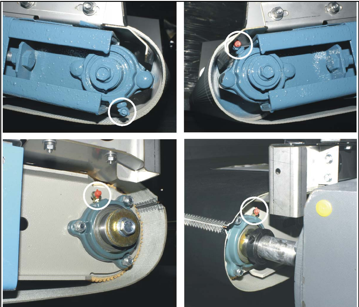
Figure 7: Grease Ports for End Roller Bearings. These are examples. Your machine can look different. All conveyor belts have four end roller bearings with grease ports.
