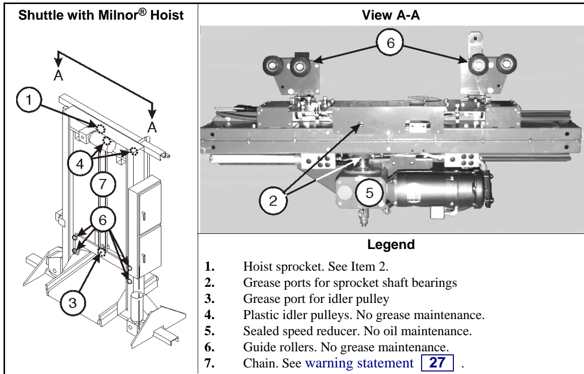
Figure 10: Elevator Maintenance—Milnor® Hoist
