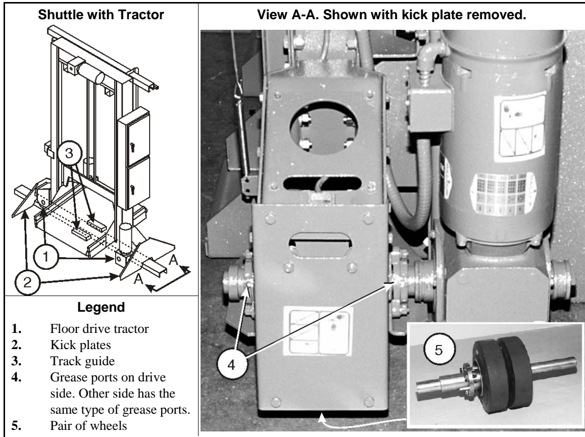
Figure 9: Tractor Maintenance All floor drive tractors have two pair of wheels. Each pair of wheels has two shaft bearings with grease ports.
